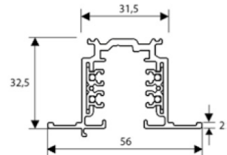
XTSCF - RECESSED
