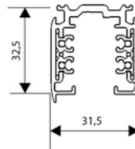
XTSC - SURFACE
